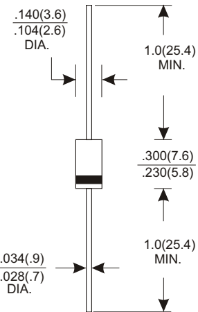
DO-15
