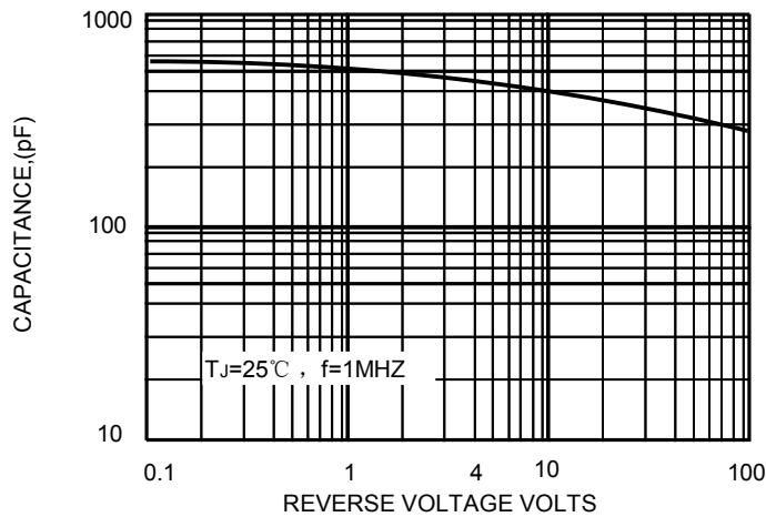
FIG.5-TYPICAL JUNCTION CAPACITANCE
